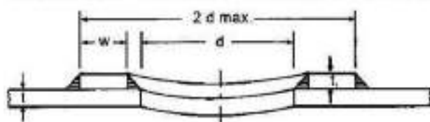
WELDS AND COMPENSATION FOR MANHOLES AND BRANCHES
