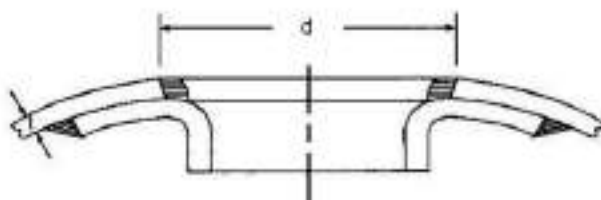
Fig. 10/11: Elliptical Manhole Flanged Frame Welded to Shell
