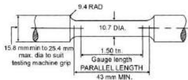
Fig. 2/3: TENSILE TEST SPECIMEN
