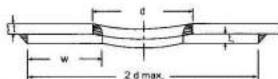
WELDS AND COMPENSATION FOR MANHOLES AND BRANCHES
