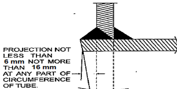
FIG. XII/34 — FUSION WELDS OF CROSS TUBES
