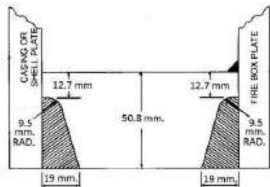
Fig. 12/37: Foundation Rings
