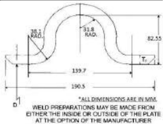
Fig. 12/31: Bowling Hoop
