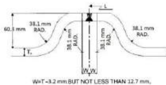
Fig. 12/33: Detail Flue Joint
