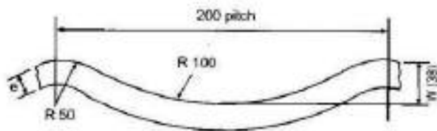
FIG. D — MORRISON TYPE FURNACES (200 MM CORRUGATION AND 38 MM DEPTH)
