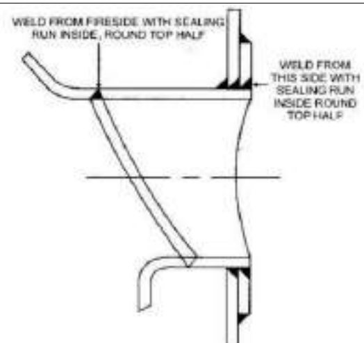
Fig. 12/41: Firehole Mouthpiece
