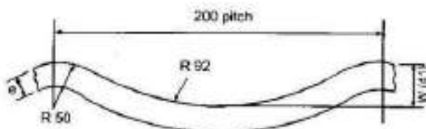
FIG. E — MORRISON TYPE FURNACES (200 MM CORRUGATION AND 41 MM DEPTH)
