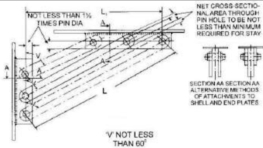
Fig. 12/103: Typical Details for Diagonal Stays (Chain Lines Indicates Stay with Multiple Links)
