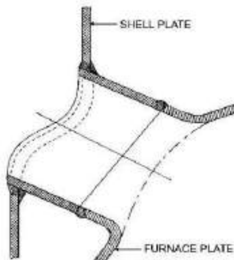
Fig. 12/44: Throat Piece
