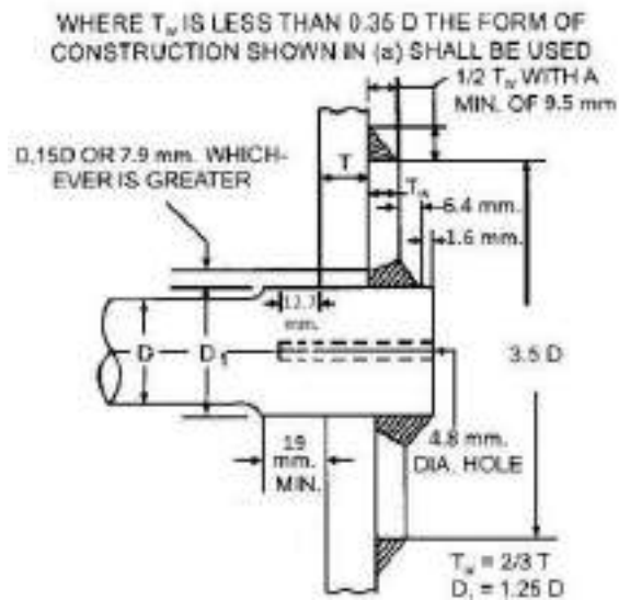
Fig. 12/55 : Attachment of Bar Stays
