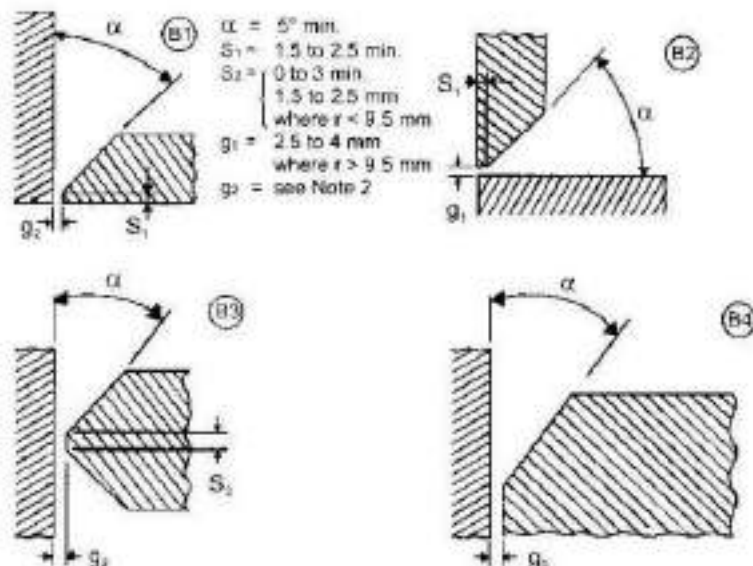
Fig. 12/108: Set in Branches (Full Penetration Weld)
