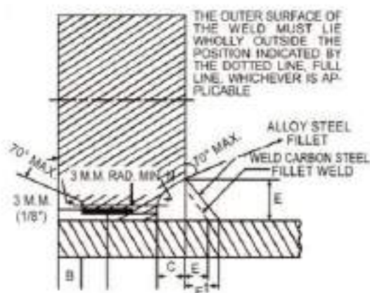
FOR CLEARANCE BETWEEN FLANGE BORE AND O.D. OF PIPE (SEE REGN. 253.2)
