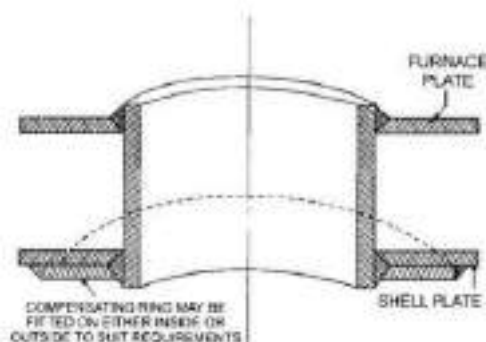
Fig. 12/40: Firehole Mouthpiece
