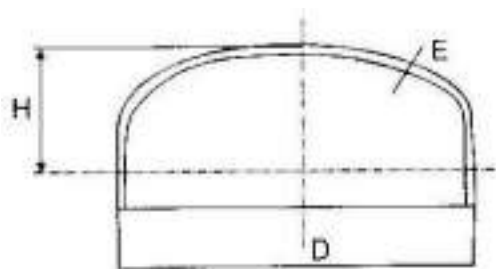
Fig. 4/16: Elliptical Head
