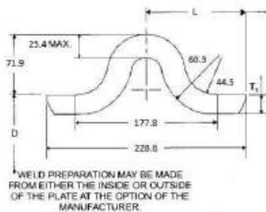
Fig. 12/32: Bowling Hoop
