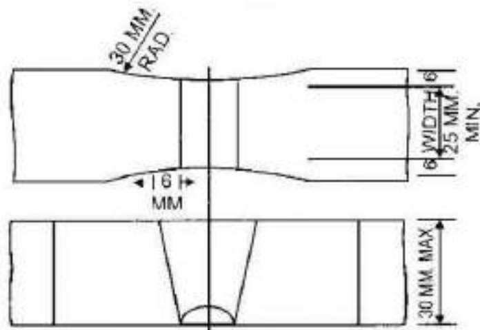
Fig. 12/73: Specimen 1A – Reduced Section Tensile Specimen All dimensions are in mm.
