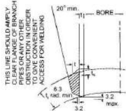
Fig. 4/32: Welded in Stand Pipe or Branch
