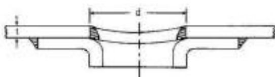
Fig.10/9: External Compensating Ring
