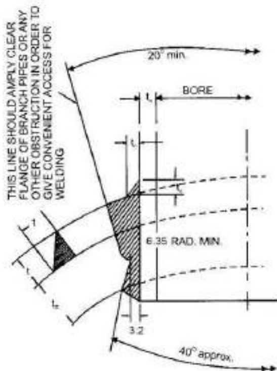
Fig. 4/30: Welded in Stand Pipe or Branch with Compensating Ring
