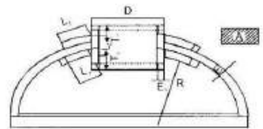
Fig. 4/20: Reinforced opening
