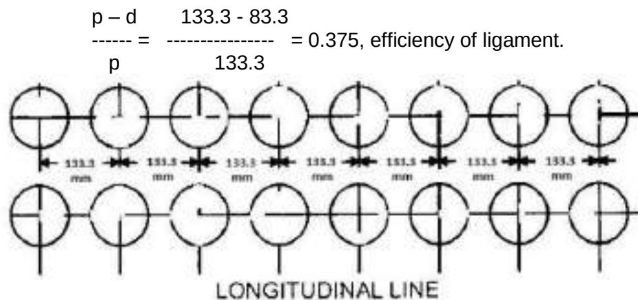
Fig. 4/8 – EXAMPLE OF TUBES SPACING WITH PITCH OF HOLES EQUAL IN EVERY ROW
