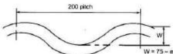
FIG G — FOX TYPE FURNACES (200 MM CORRUGATION AND 75 MM DEPTH)
