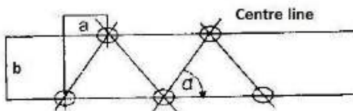
Fig. 4/15: Regular Saw-Tooth Pattern of Holes
