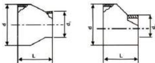
CONCENTRIC REDUCER
