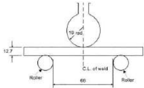
Fig. 2/8: Method of Carrying Out Bend Tests
