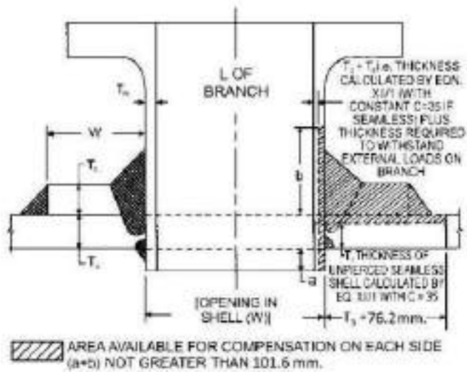
Fig. 12/80: Compensation for Branch
