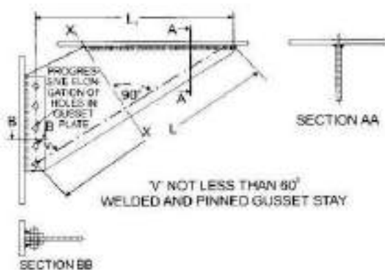
Fig. 12/102: Typical Details for Welded and Pinned Gusset Stay
