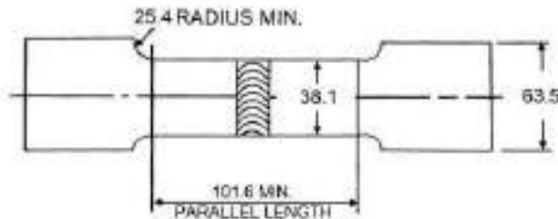
Fig. 2/7: Dimensions of Transverse Tensile Test Specimen
