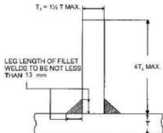
Fig. 12/29: Plain Bar
