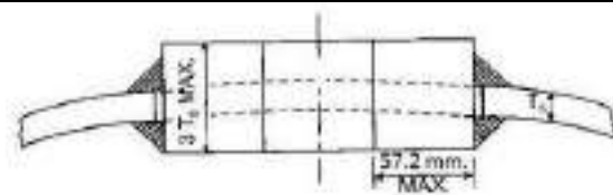
Fig. 12/115: Pads Welded on For Studs
