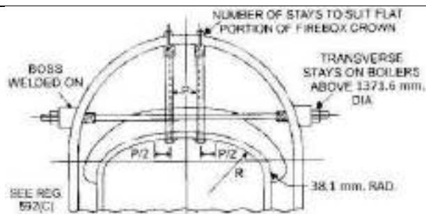
Fig. 12/95: Arrangement of Firebox Crown and Transverse Stays for Locotype Boilers
