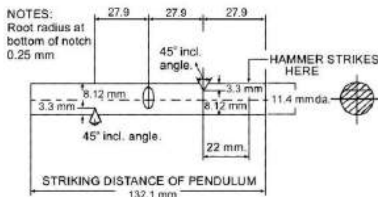
Fig. 2/4: IMPACT TEST SPECIMEN
