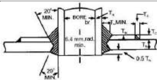
Fig. 12/111: Minimum Weld Attachment For Stand Pipes Over 127 mm Bore Requiring Compensation Plates
