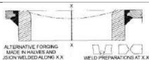
Fig. 12/65: Fusion Welded Oval Manhole Frame
