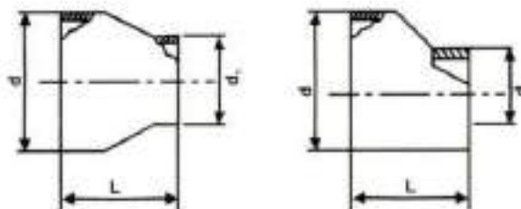
CONCENTRIC REDUCER
