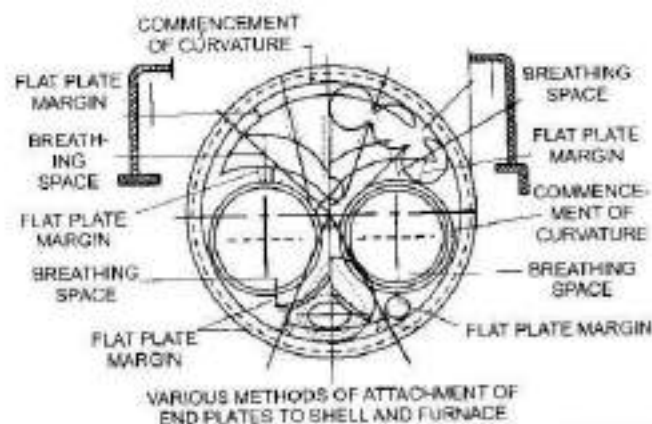
Fig. 12/86: Typical Arrangement of End Plates on Lancashire Boilers
