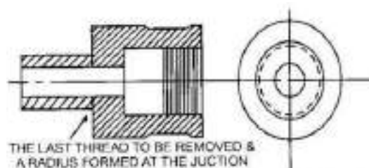
Fig. 12/70: Typical Mild Steel Distance Piece for Mountings
