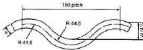
FIG C — FOX TYPE FURNACES (150 MM CORRUGATION AND 41 MM DEPTH)
