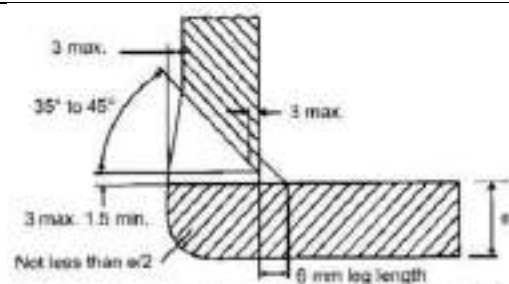
Fig. 12/16: Flue Connections to End Plates (Dished or Flat)
