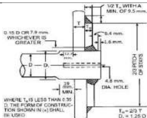
Fig. 12/59: Attachment of Bar Stays
