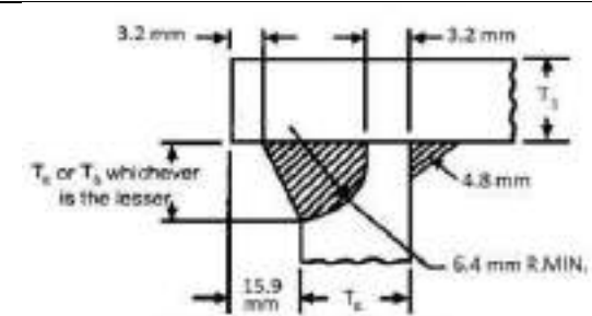
Fig. 12/12: Flat End
