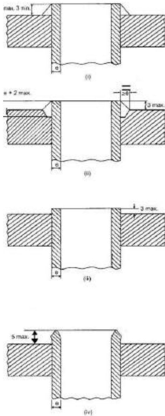
Fig. 12/82: Typical Attachment of Plain Tubes
