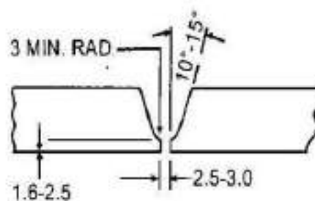
Fig. 7/25: Single U for Use Without Backing Ring
