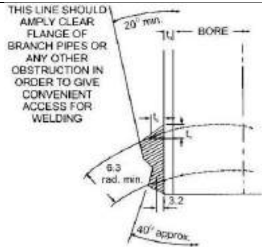
Fig. 4/31: Welded in Stand Pipe or Branch
