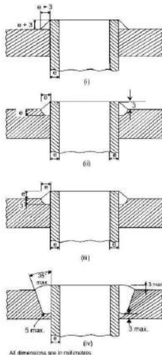
Fig. 12/84: Typical Attachment of Stay Tubes
