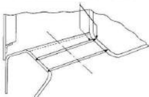
Fig. 12/43: Welding of Flue Pipes
