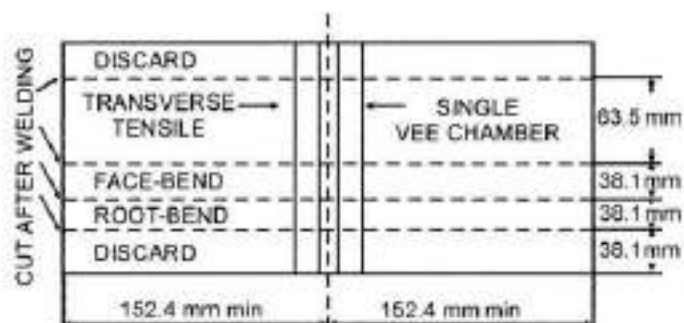
Fig. 2/5: METHOD OF MAKING TRANSVERSE TENSILE AND BEND TEST SPECIMENS
