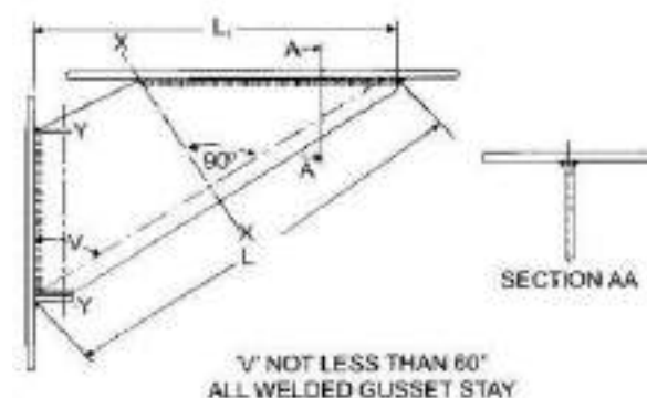
Fig. 12/101: Typical Details For All-Welded Gusset Stay
