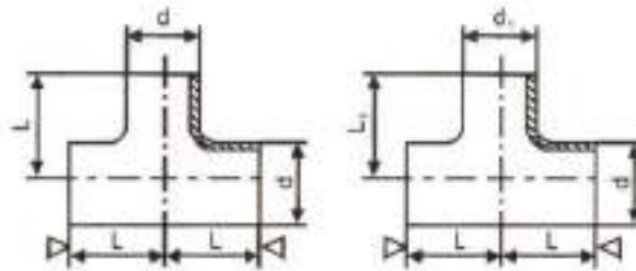
EQUAL TEE
