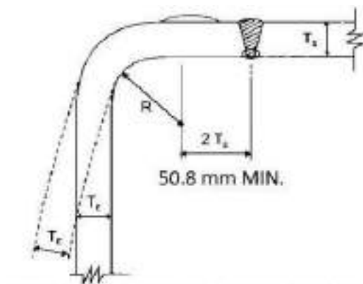
Fig. 12/9: Flanged End Plates Ends Thicker Than Shell
