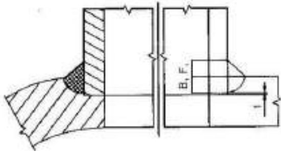
Fig. 4/35: Unreinforced Branches Inaccessible for Welding Inside Shell
