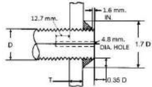
Fig. 12/48: Attachment of Firebox and Combustion Chamber Stays
