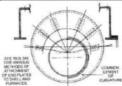
Fig. 12/88: Typical Arrangement of End Plates on Cornish Boilers
