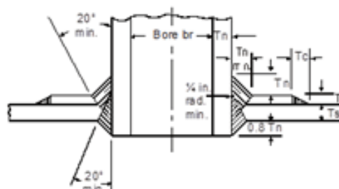
Fig:10/22, 10/23, 10/24 — MINIMUM WELD ATTACHMENTS FOR STANDPIPES OVER 5 IN. BORE NOT REQUIRING COMPENSATING PLATES. Fig:10/25 — MINIMUM WELD ATTACHMENT FOR STANDPIPES OVER SURFACE REQUIRING COMPENSATING PLATES
