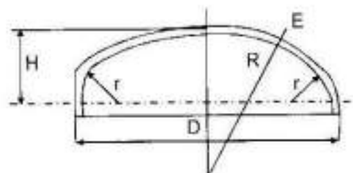
Fig. 4/17: Torispherical Head
