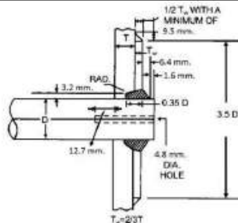
Fig. 12/52: Attachment of Bar Stays
