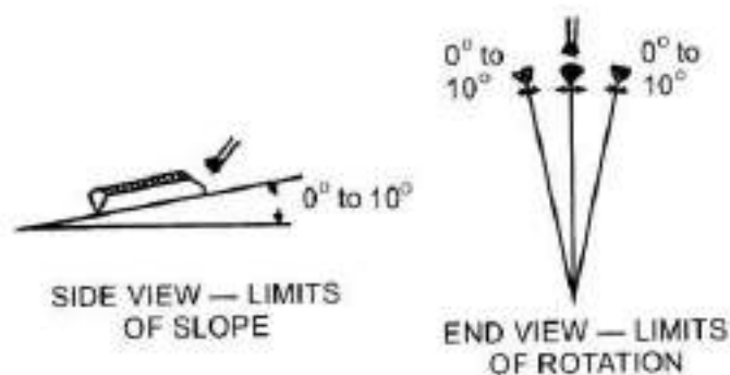
Fig. 2/12: Flat (F)
