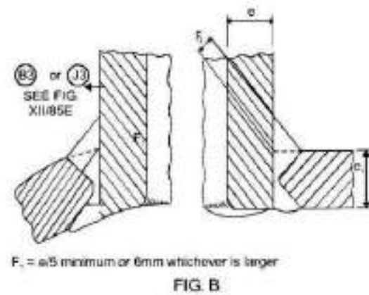
Fig. 12/108: Set in Branches (Full Penetration Weld)
