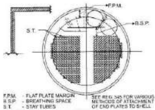
Fig. 12/93: Typical Arrangement of End Plates on Multi-Tubular Boilers
