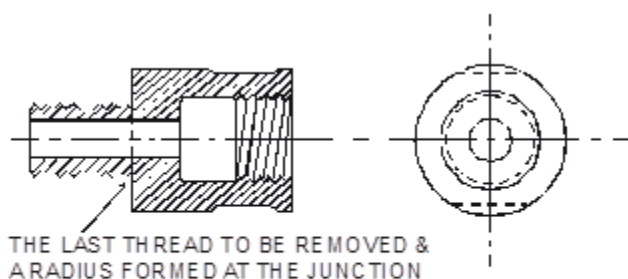
Fig. X/14: Typical Mild Steel Distance piece for Mountings
