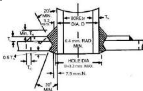
Fig. 12/112: Minimum Weld Attachment For Stand Pipes Over 127 mm Bore Requiring Compensation Plates
