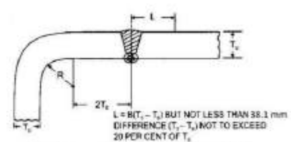
Fig. 12/10: Flanged Flat End Plates
