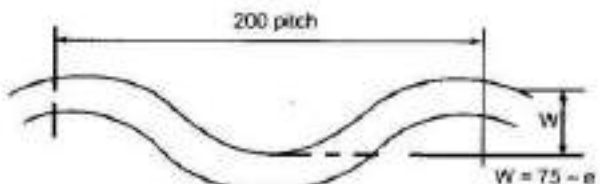
FIG. G — FOX TYPE FURNACES (200 MM CORRUGATION AND 75 MM DEPTH)
