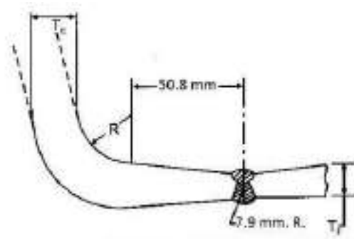
Fig. 12/16: Flue Connections to End Plates (Dished or Flat)
