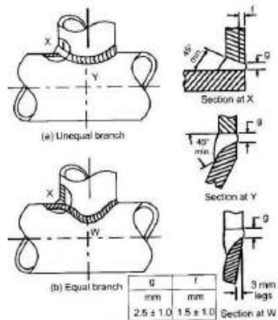
Fig. 12/118: Typical Preparation and Assembly of Set on Right Angle Branches Without Backing
