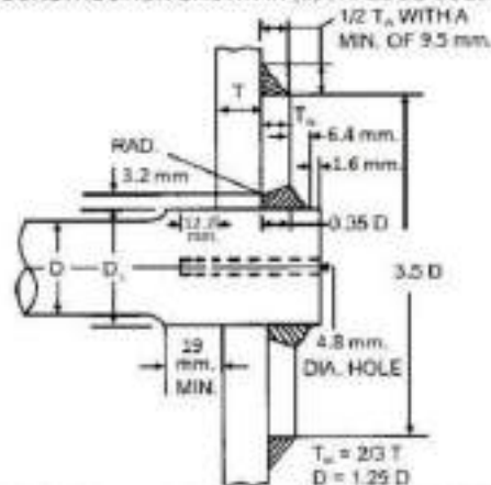
Fig. 12/54: Attachment of Bar Stays
