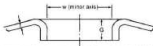
Fig. 10/10: Internal Compensating Ring
