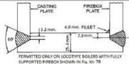
Fig. 12/37: Foundation Rings
