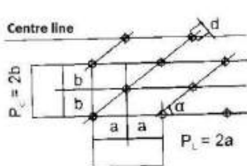
Fig. 4/13: Regular Staggering of Holes
