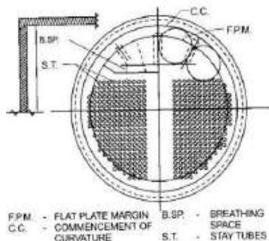
Fig. 12/92*: Typical Arrangement of End Plates on Cornish Boilers
