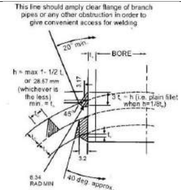
Fig. 4/27: Welded in StandPipe or Branch with Compensating Ring For StandPipes and Branches up to and including 101.6 mm Bore
