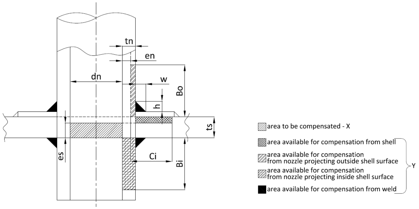
Fig. 4/22: Compensation of Set through branch openings
