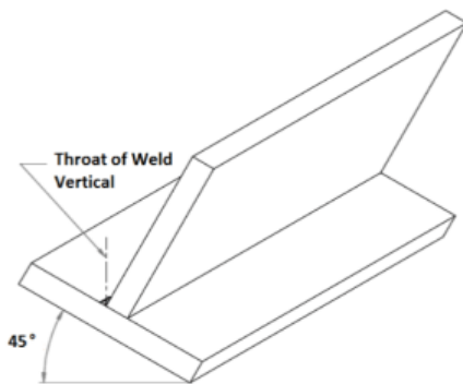
FIGURE13/LFF: Plate Fillet Flat Position
