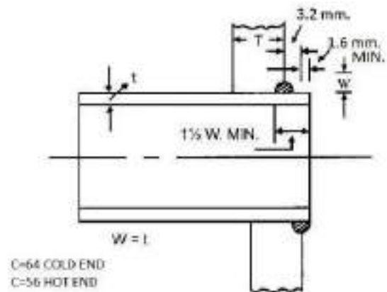
Fig. 12/83: Tubes to be Lightly Expanded into the Plate Before Welding
