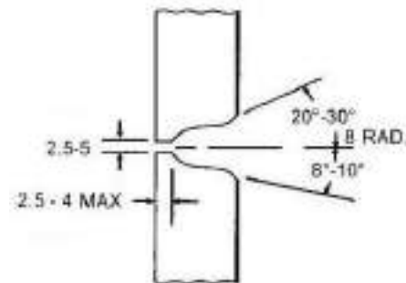
Fig. 7/20: U-Groove for Use With Oxy-Acetylene Base Run
