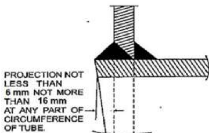
Fig. 12/42 — FUSION WELDS OF CROSS TUBES
