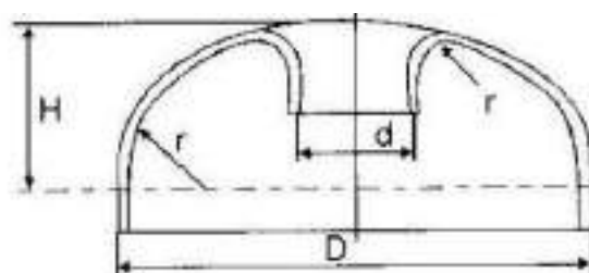
Fig. 4/18: Head with Manhole (Elliptical or Torispherical)
