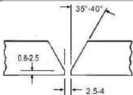
Fig. 7/23: Plain Vee for Use Without Backing Ring
