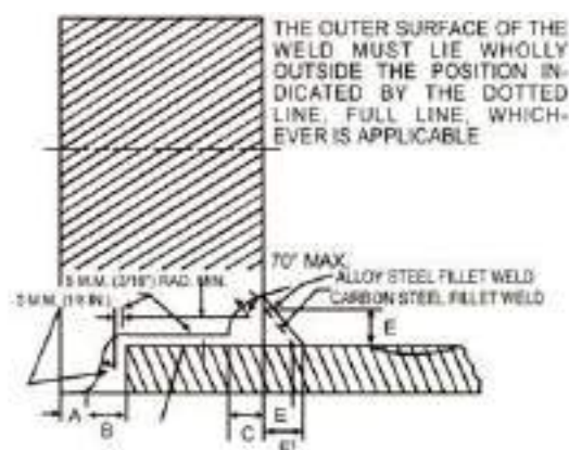
FOR CLEARANCE BETWEEN FLANGE BORE AND O.D. OF PIPE [SEE REGN. 263(2)]
