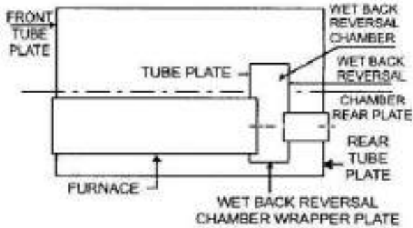
Fig. 12/26: Wet Back Boiler
