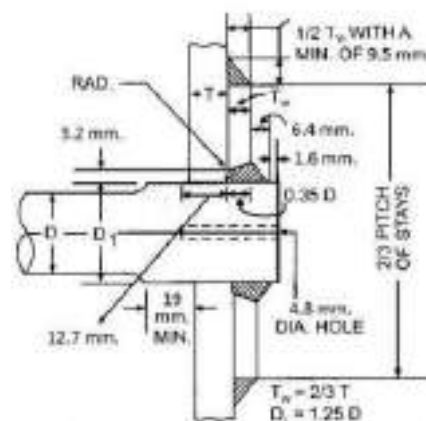
Fig. 12/58: Attachment of Bar Stays
