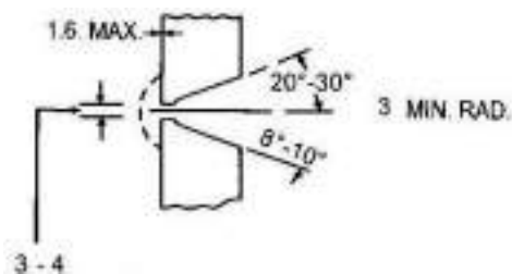
Fig. 7/14: Permissible Alternative Preparation for Vertical or Nearly Vertical Pipe U-Groove for Use with Backing Ring
