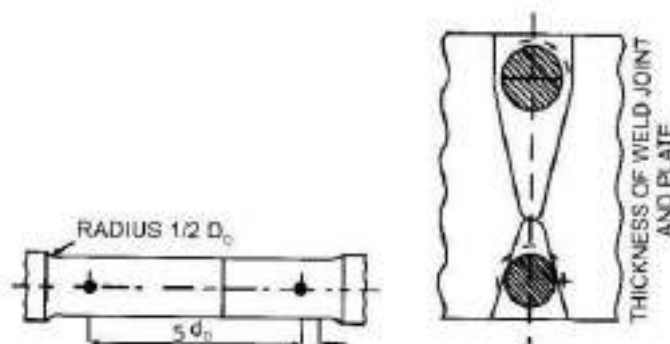
Fig. 4/4: Reduced Section Tensile Specimen in Thick Plate
